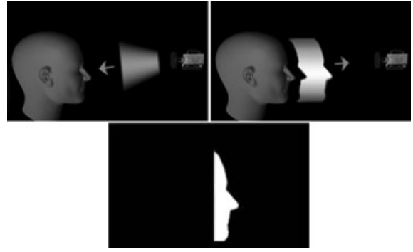
Figure 2: The shutter principle: A 'light wall' is emitted from the camera (top-left) and reflected by the object (top-right). Gating the reflected optical signal yields distance-related portions of the 'light wall', which are measured in the CCD pixels [IY01].
