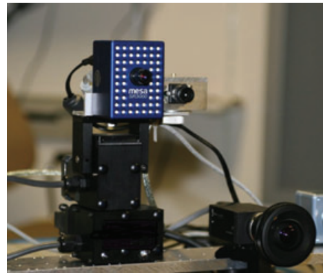
Figure 6: Setup consisting of a ToF camera (SwissRanger 3000) mounted together with a CCD firewire camera on a pan-tilt unit and a fisheye camera mounted at the bottom right.
