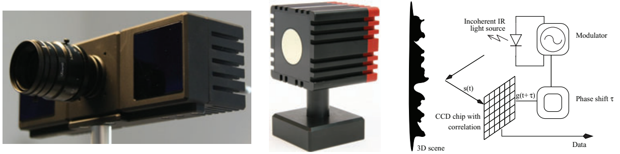
Figure 1: Left: PMDTec/ifm electronics CamCube camera. Middle: MESA SR4000 camera. Right: The ToF phase-measurement principle.
