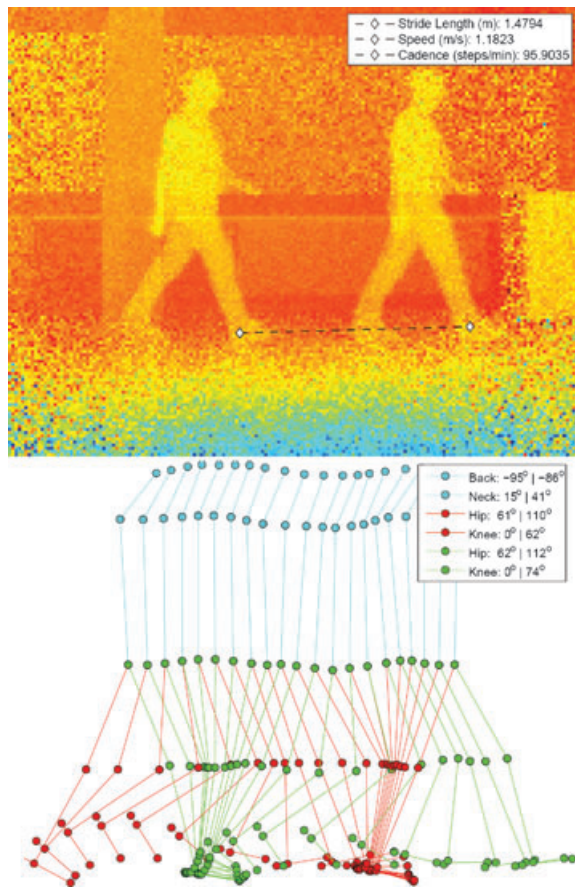
Figure 11: Top: An overlay of two ToF images in a gait sequence. The two images correspond to one stride. Bottom: The articulated human pose model fitted to the ToF gait sequence using a pose-cut algorithm for ToF data [RPL09].
