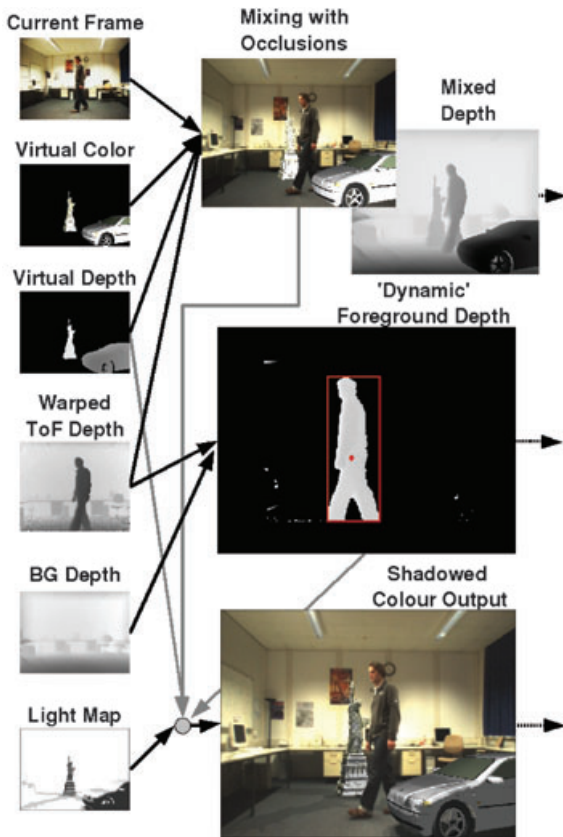
Figure 9: Overview of the colour mixing and shadow casting of real and virtual objects on the GPU. On the left hand side, all the input images are displayed. Based on the difference depth images, mutual occlusions can be handled in the augmentation. Moreover, foreground-segmented depth images and mixed depth images are delivered. The scaling of the augmented image via the light map yields the final colour image output (from [SBK*08a]).
