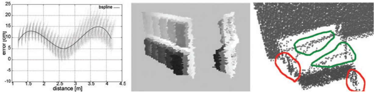
Figure 3: Error sources of PMD-based ToF cameras. Left: Systematic distance error for all pixels (grey) and fitted mean deviation (black). Middle: Intensity-related distance error when sensing a planar object with varying reflectivity. Right: Motion artefacts (red) and flying pixels (green) for a horizontally moving planar object in front of a wall.
