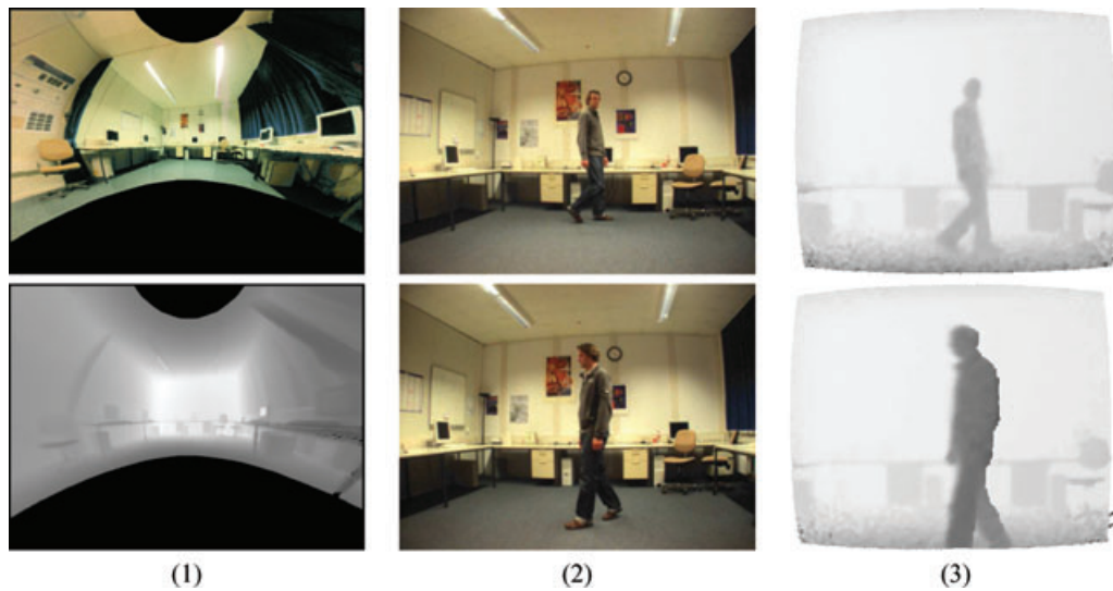
Figure 8: Column (1): The texture and the depth image (dark = near, light = far) as a panorama after scanning the environment. For visualization, the panorama is mapped onto a cylindric image. Columns (2) and (3): Two images out of a sequence of a person walking through the real room with a virtual occluder object. (2): Original image; (3): ToF depth image for depth keying.
